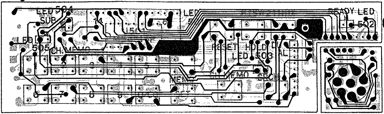
Component side
