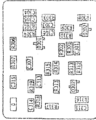
(A103) PTB172 Component Side View
