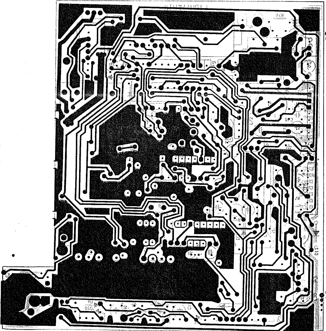
(A101) PTB172 Component Schematic Side
