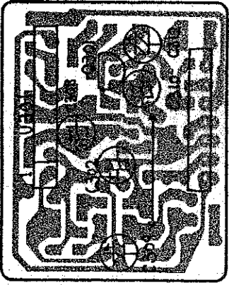
(APO3) APT221/3 Component Side View
