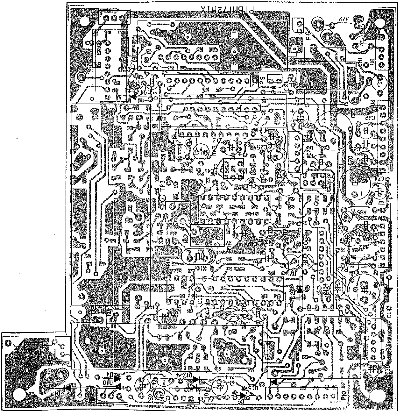
(AP01) PTBM 172 Component Side View
