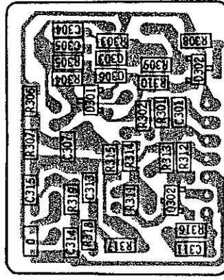
(AP03) APTZZ113 Component Side View
