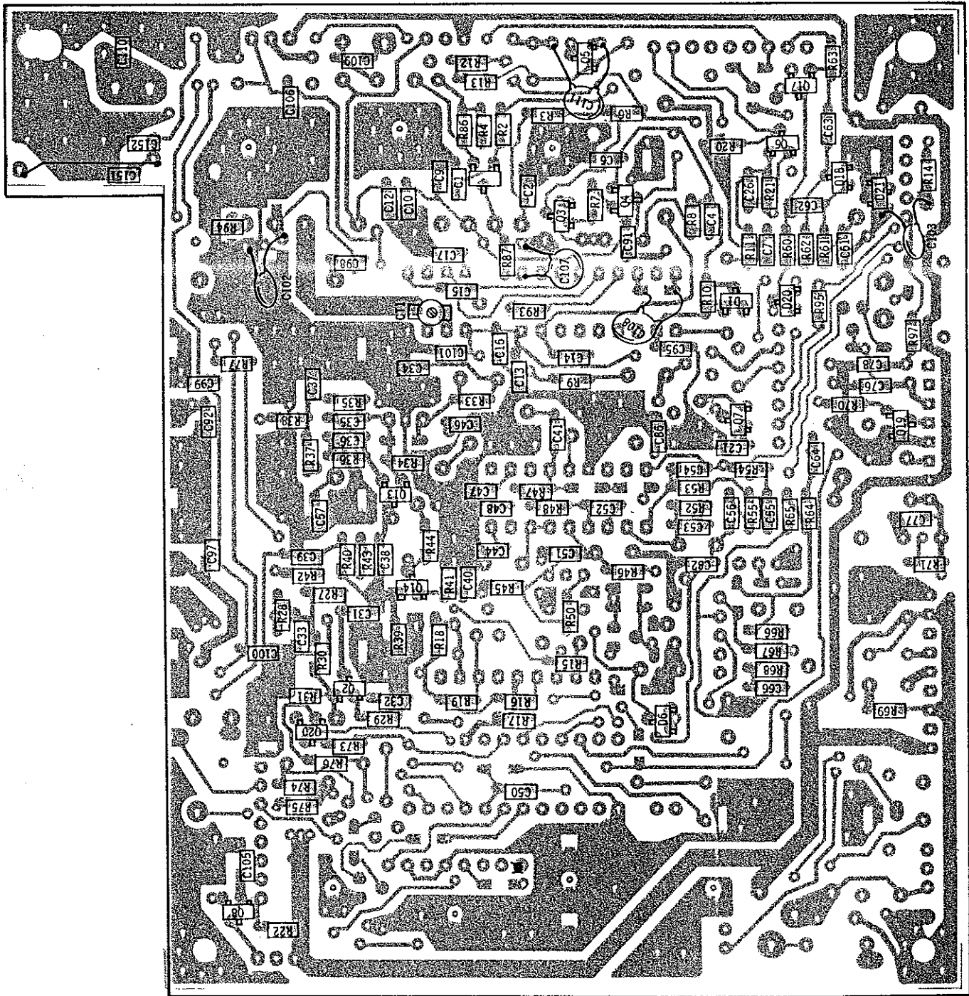
(AP01) APTBM172 Chip parts location
